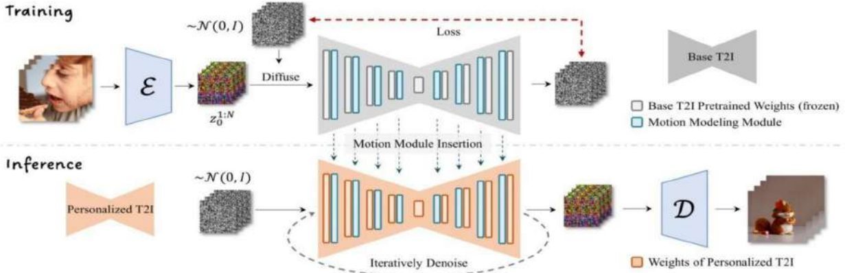
Fig1. Shows the AnimateDiff pipeline. Given a foundation T2I model (for example, Stable Diffusion [22]), we train a motion modeling module on video datasets to encourage it to distill motion priors. Only the parameters of the motion module are modified at this step, keeping the feature space of the underlying T2I model. Once trained, the motion module can transform any personalized model based on the basic T2I model into an animation generator, then generate various and personalized animated visuals via an iterative denoise process.
