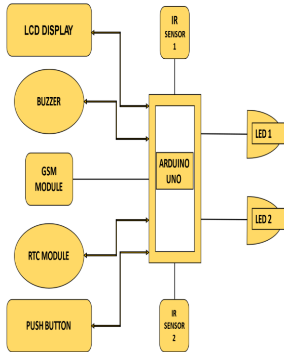
Figure 1Block Diagram
